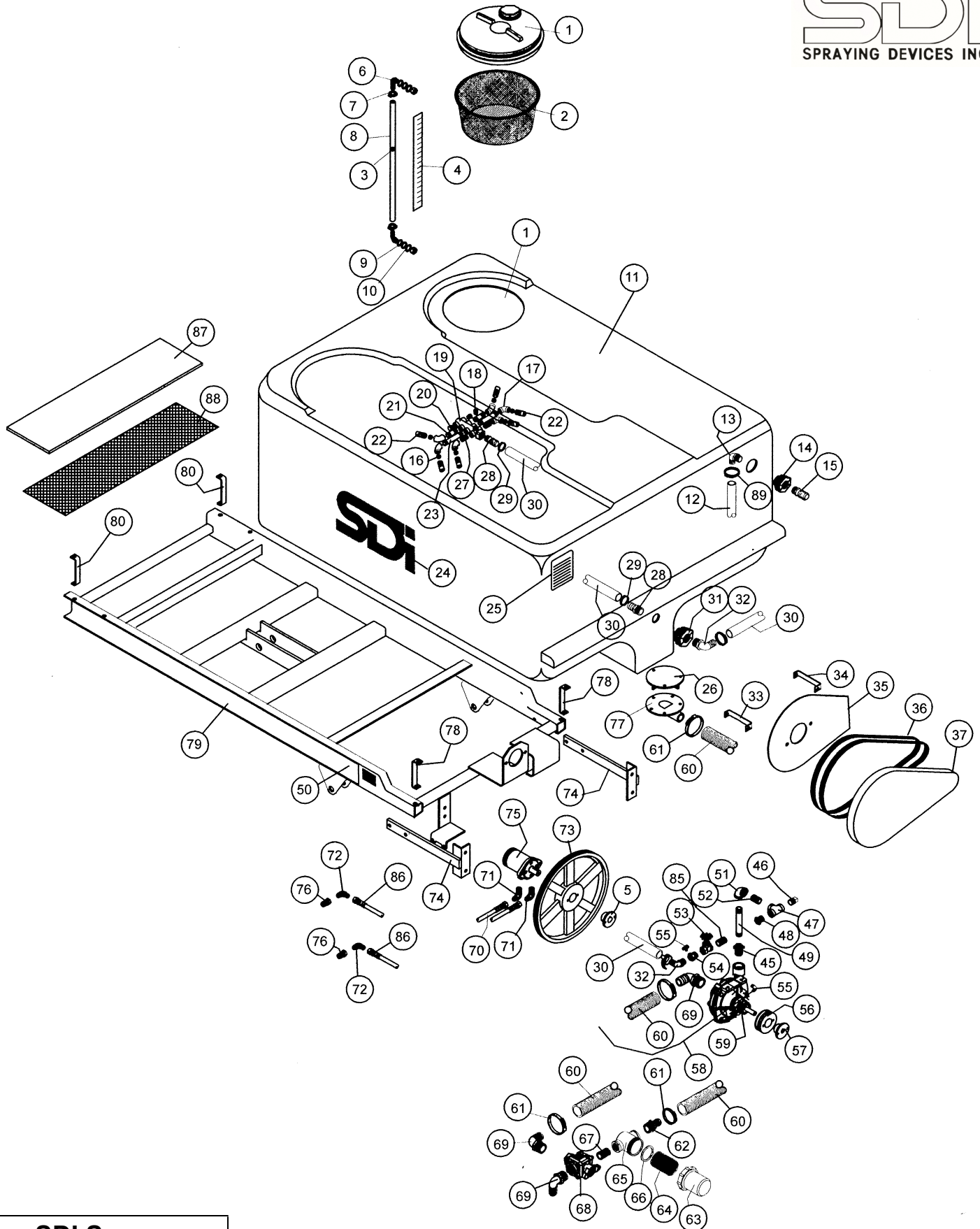
SDI Sprayer Model XD300CA
