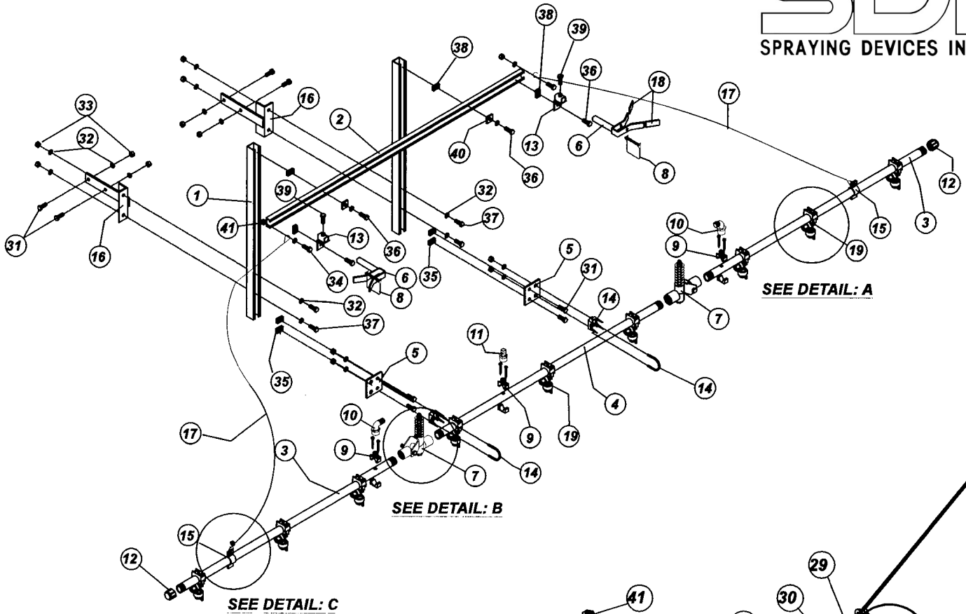
SEE DETAIL: C
