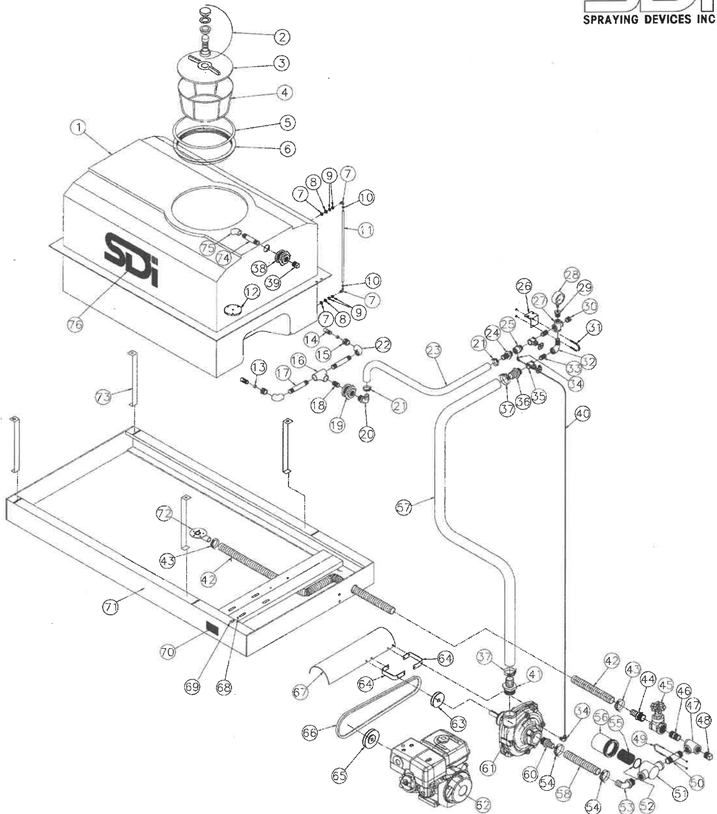
SDI Sprayer Model 300-65H6J
